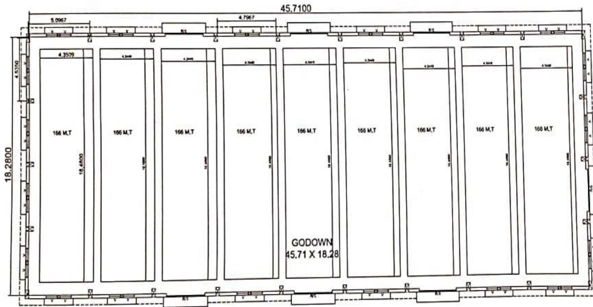
GODOWN PLAN scale 1:100
